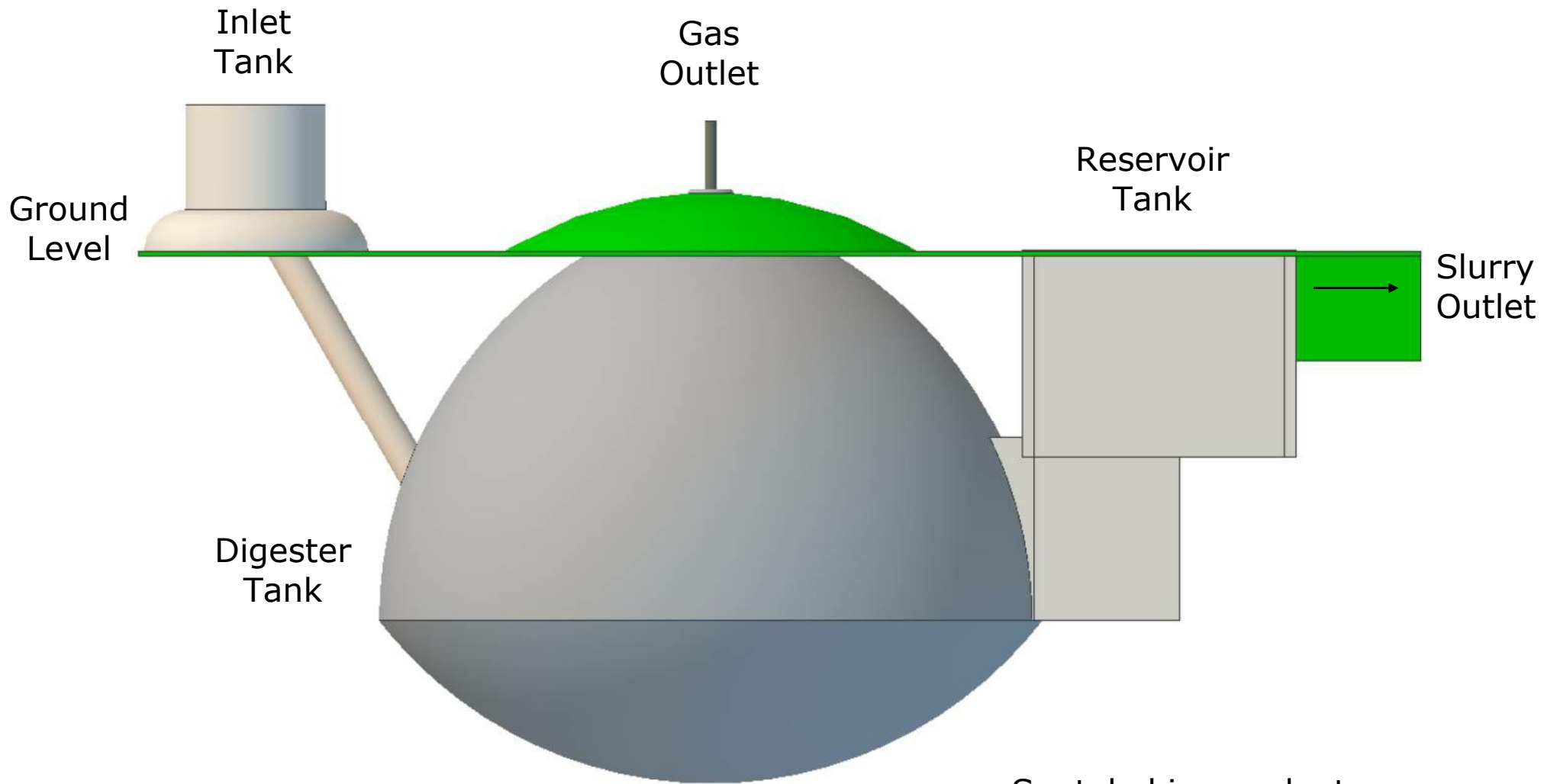
Suntala biogas plant
